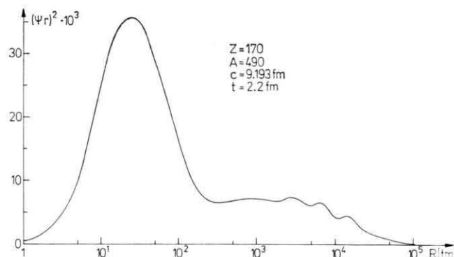
Fig. 6. The total radial density |\psi r|^2 of Z = 170 . Observe the big principal maximum in comparison with those atoms with lower Z which are shown by Fricke and others 9 . Note half logarithmic scale.
